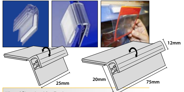
Hinged flip strip with adhesive.
