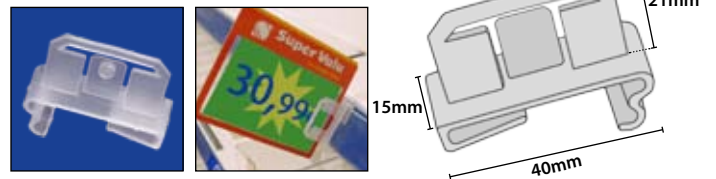
Shelf edge poster bracket for data strip.
